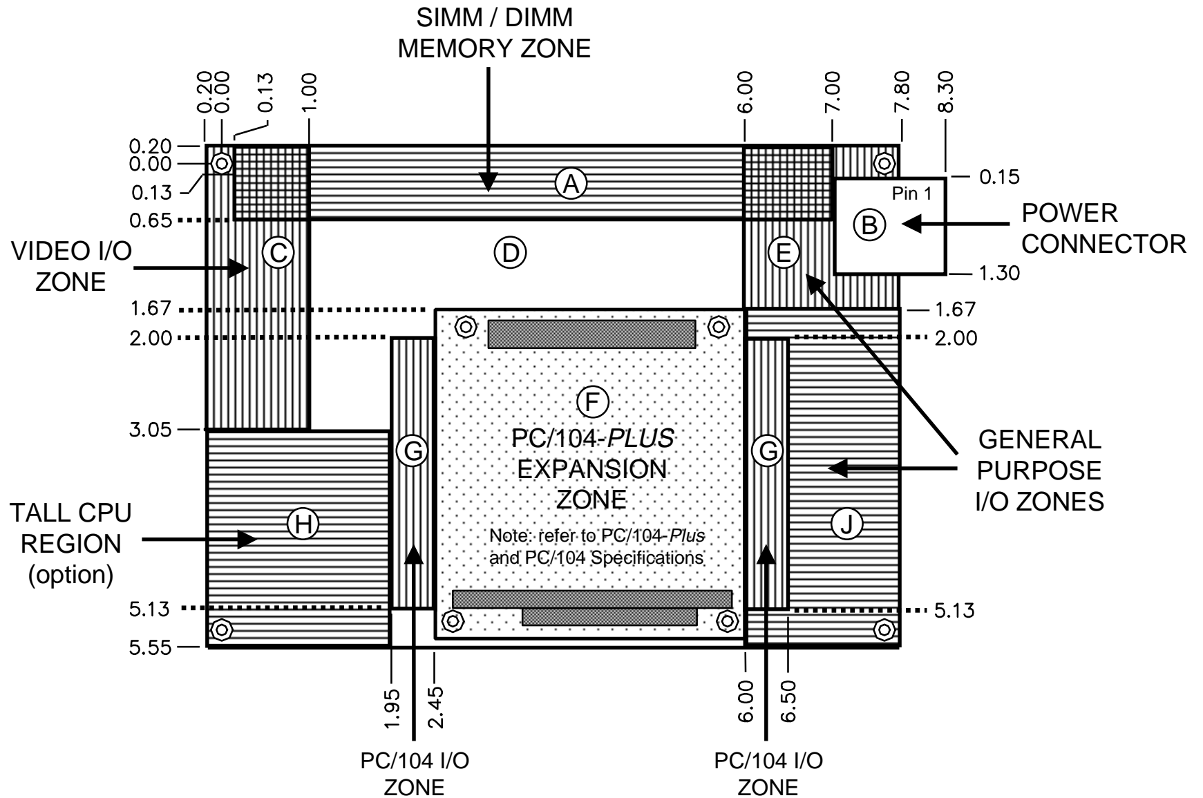
Figure 2. EBX Component Zones, Tall CPU Option
