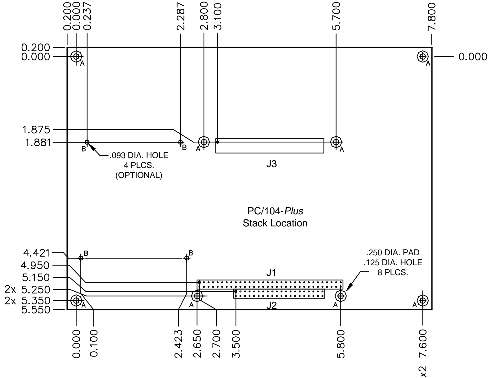
Figure 1. EBX Detailed Mechanical Dimensions
