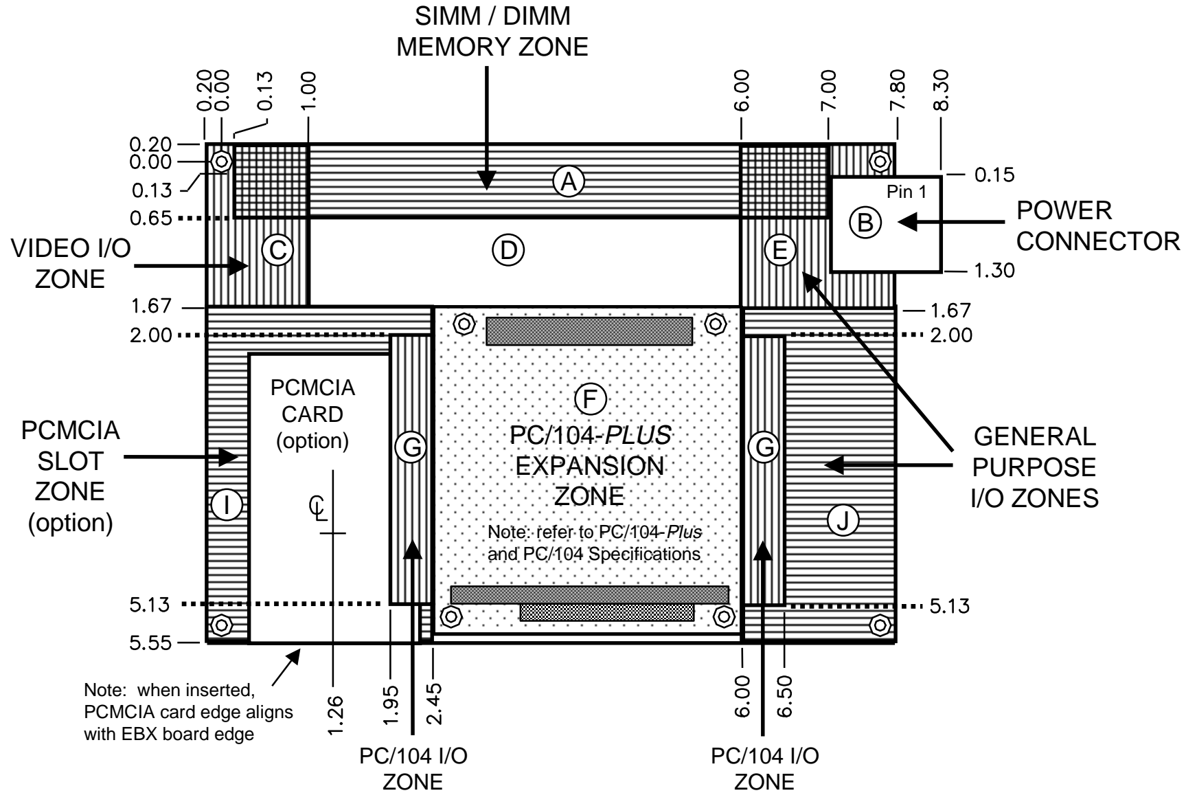
Figure 3. EBX Component Zones, PC Card Slot Option
